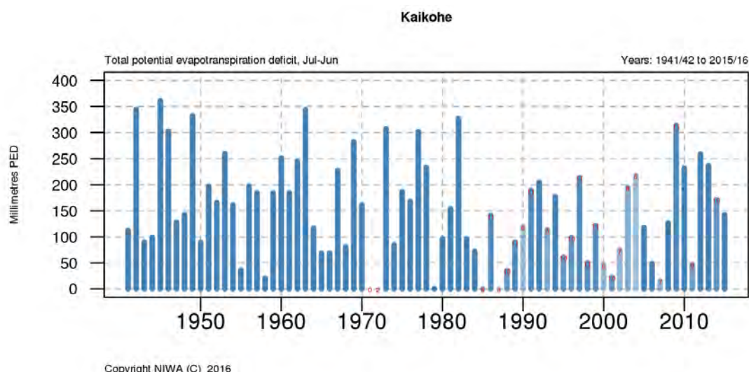
Figure 4-8: PED accumulation from 1941-2015 (July-June years) for Kaikohe (combined record from agent numbers 1126, 1129, 1134). Light blue bars indicate years where there are missing data, and small red numbers indicate the amount of months in that year with full data. © NIWA.
