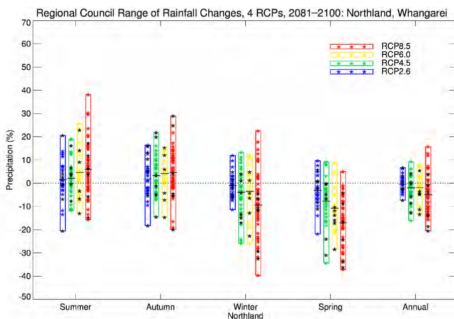
Figure 5-18: Projected seasonal rainfall changes by 2090 (2081–2100) for Whangarei, for the four RCPs. The vertical coloured bars show the range over all climate models used, and coloured stars the projected changes for each model individually (results from statistical downscaling). The black stars represent the 6-model dynamical downscaling changes. The short horizontal line is the model-average rainfall over all statistical and dynamical models. Blue = RCP 2.6, 23 models; green = RCP 4.5, 37 models; yellow = RCP 6.0, 18 models; red = RCP 8.5, 41 models. © NIWA.
