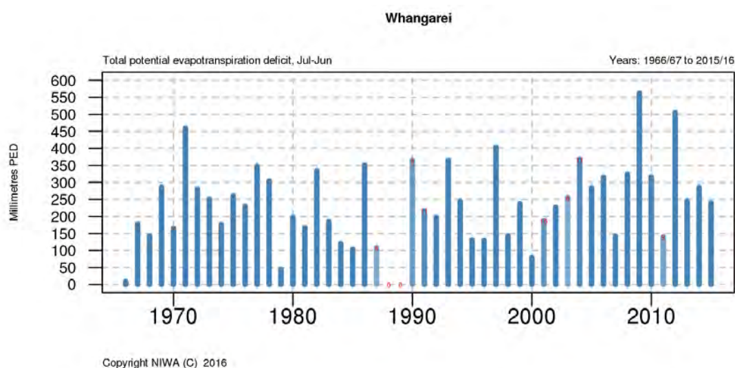
Figure 4-5: PED accumulation from 1966-2015 (July-June years) for Whangarei (combined record from agent numbers 1283 and 1287). Light blue bars indicate years where there are missing data, and small red numbers indicate the amount of months in that year with full data. © NIWA.
