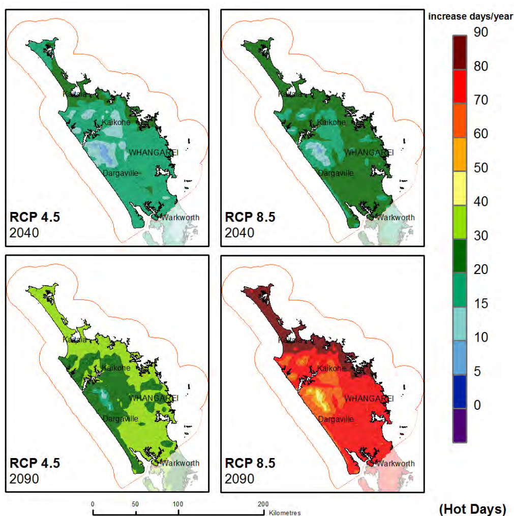
Figure 5-8: Projected increase in number of hot days per year ( T_{max} > 25^{\circ}\text{C} ) at 2040 & 2090 for RCP 4.5 (left panels) and RCP 8.5 (right panels), for Northland Region. Projected change in hot days is relative to 1986-2005. The numbers on the scale refer to the increase in the number of hot days, e.g. the north-east coast of Northland is projected to experience an increase in the number of hot days by 80-90 days by 2090 under RCP8.5 (lower right panel). © NIWA.
