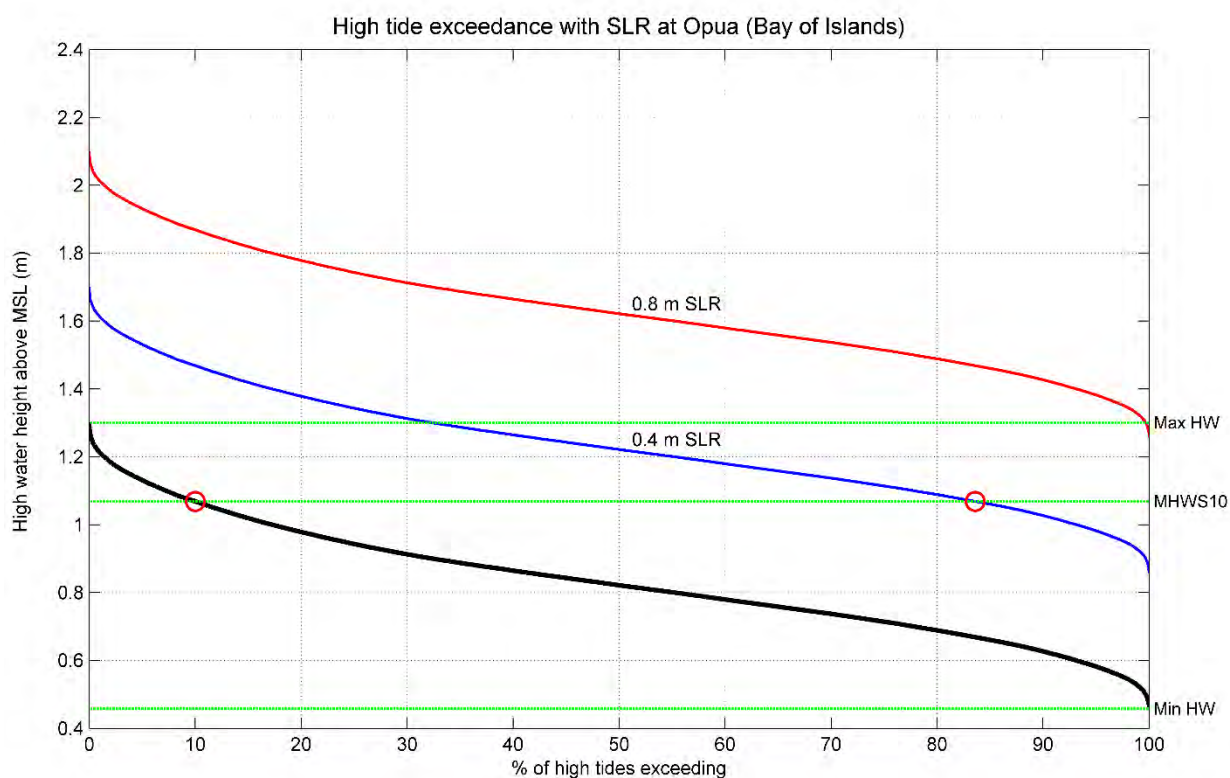
Figure 5-29: The frequency of occurrence of high tides exceeding different present day tide marks at Opua, Bay of Islands. The tide marks for the present is shown by the heavy line, 0.4m of sea-level rise (blue line) and 0.8m of sea-level rise (red line). ©NIWA.
