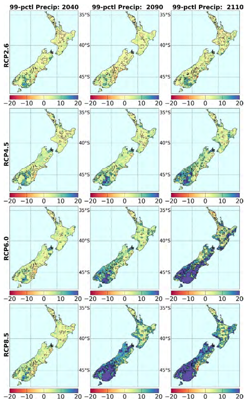
Figure 5-23: Change in the magnitude of the 99th percentile of daily precipitation (in %). For all four RCPs and three future time periods, relative to the daily 99th percentile in the baseline 1986-2005 period. The red colours indicate a decrease in extreme rainfall, orange little change, and green, blue, and purple a progressive increase in extremes. After Mullan et al. (2016).
