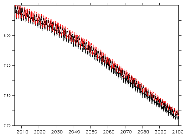
Figure 5-31: Projected mean surface pH for the NZ EEZ open ocean from a suite of six CMIP5 models, using the RCP8.5 scenario. The outputs from the models that show the closest fit to carbonate observations in the NZ EEZ during the present period are highlighted in red (S. Mikaloff-Fletcher, NIWA).
