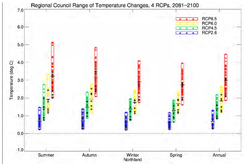
Figure 5-16: Projected seasonal temperature changes by 2090 (2081–2100) averaged over the Northland Region, for the four RCPs. The vertical coloured bars show the range over all climate models used, and coloured stars the projected changes for each model individually (results from statistical downscaling). The black stars represent the 6-model dynamical downscaling changes. The short horizontal line is the model-average warming over all statistical and dynamical models. Blue = RCP 2.6, 23 models; green = RCP 4.5, 37 models; yellow = RCP 6.0, 18 models; red = RCP 8.5, 41 models. © NIWA.
