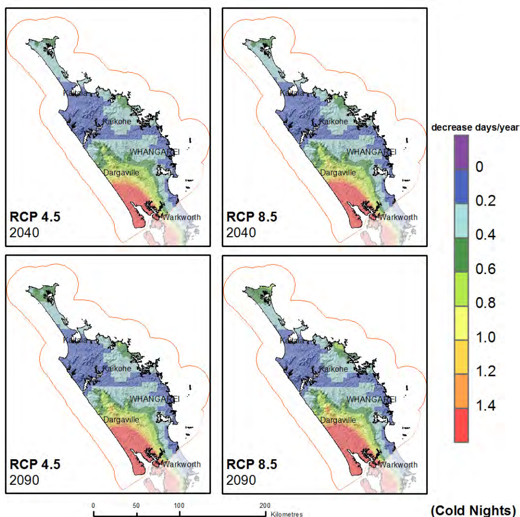
Figure 5-9: Projected decrease in number of cold nights per year ( T_{min} < 0^{\circ}\text{C} ) at 2040 & 2090 for RCP 4.5 (left panels) and RCP 8.5 (right panels). Projected change in cold nights is relative to 1986-2005. The numbers on the scale refer to the decrease in the number of cold nights, e.g. the south-west part of Northland is projected to experience a decrease in the number of cold nights by over 1.4 nights per year by 2090 under both RCP 4.5 and RCP 8.5 at 2040 and 2090. © NIWA.
