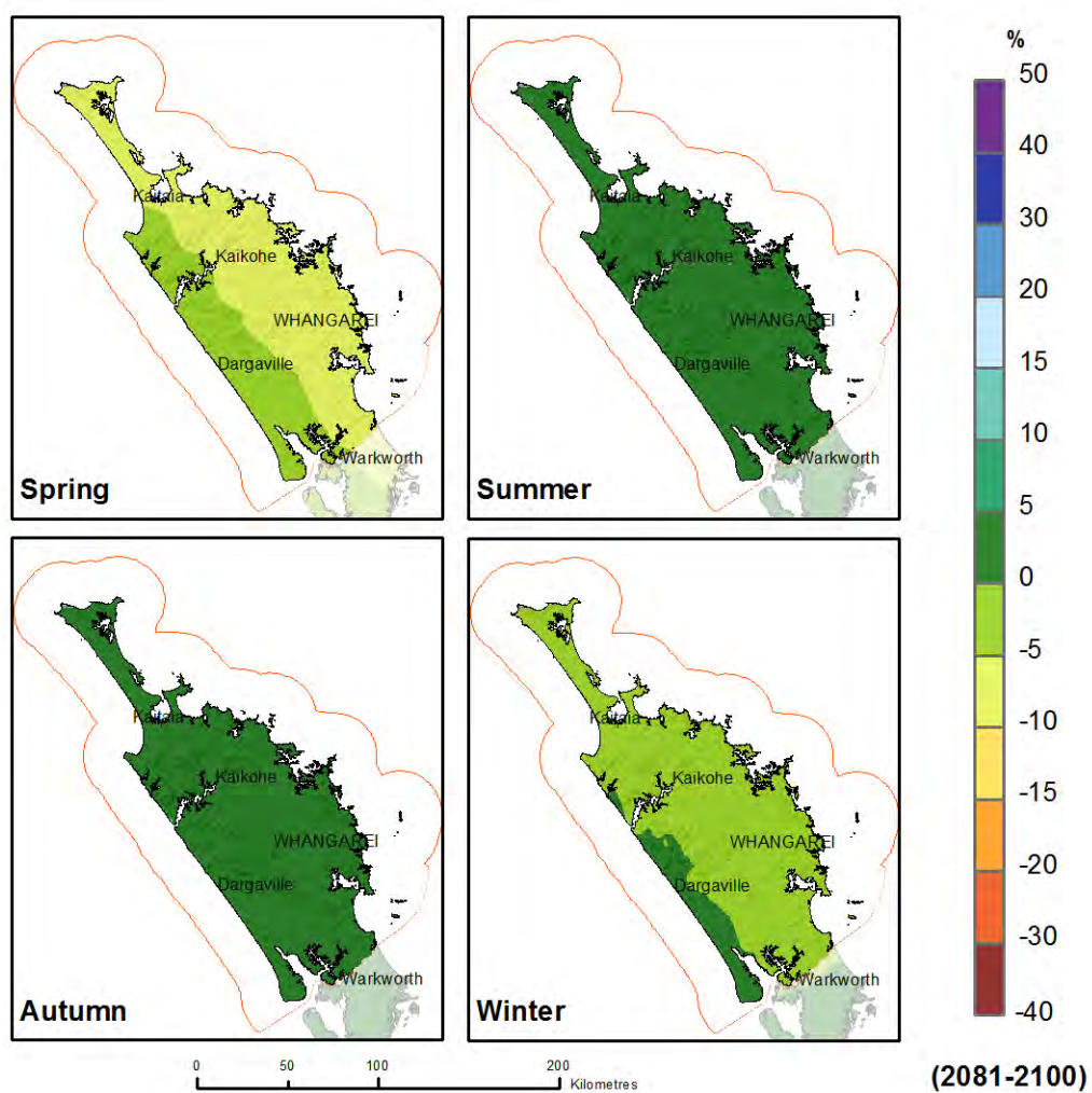
Figure 5-12: Projected seasonal precipitation changes (in %) at 2090 (2081-2100 average). Relative to 1986-2005 average, for the RCP 4.5 scenario, averaged over 37 climate models. ©NIWA.
