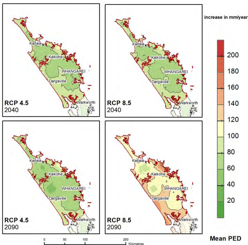
Figure 5-24: RCM-projected changes in Potential Evapotranspiration Deficit (PED, in mm accumulation over the July-June 'hydrologic year') for Northland Region. With respect to the baseline 1995 period, for RCP 4.5 and RCP 8.5, for 2040 and 2090. The black contour lines are at 40, 80, 120 and 160 mm/year intervals.
