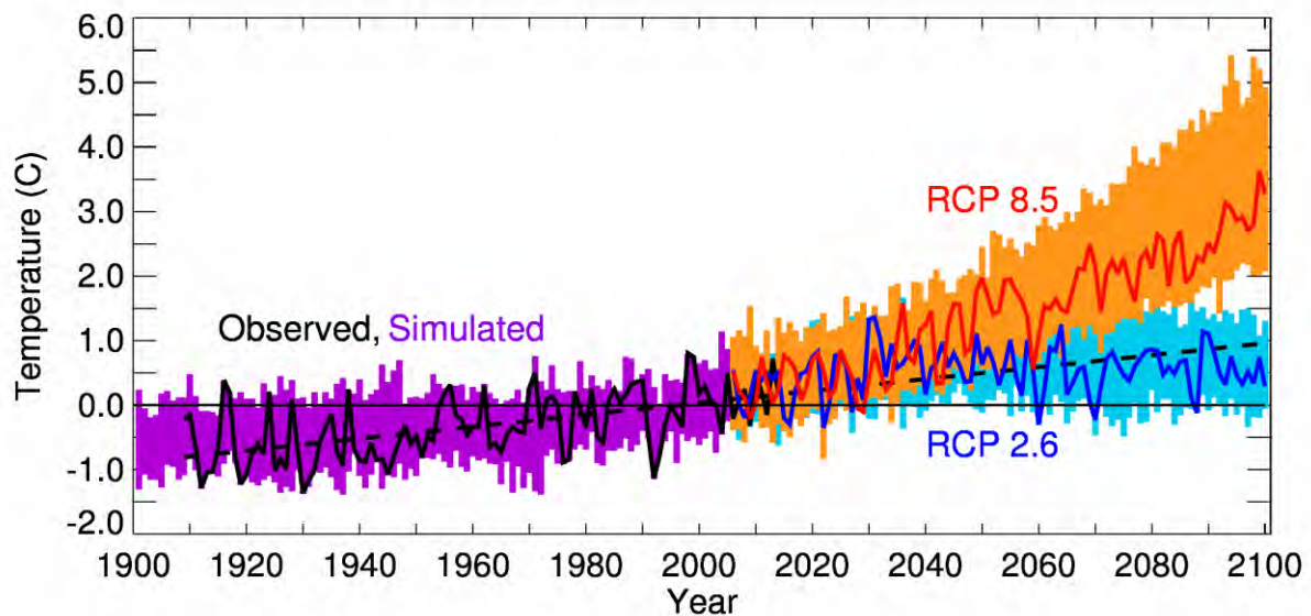
Figure 5-33: New Zealand Temperature - historical record and an illustrative schematic projection illustrating future year-to-year variability. (See text for full explanation). After Mullan et al. (2016).
