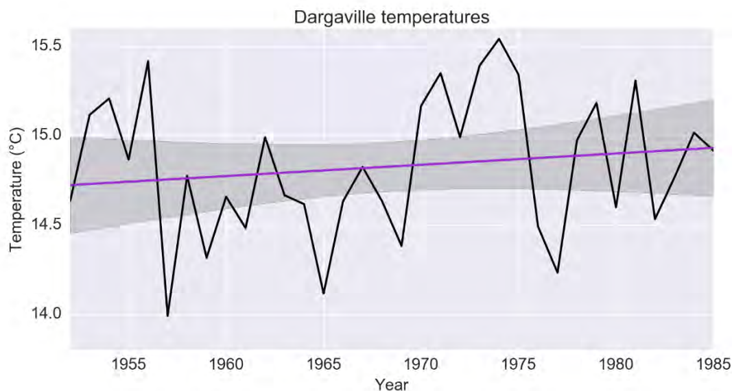
Figure 4-3: Annual mean temperature time series for Dargaville (agent number 1192) from 1951 to 1985. The purple line removes the year-to-year variability and shows a small upward trend. © NIWA.
