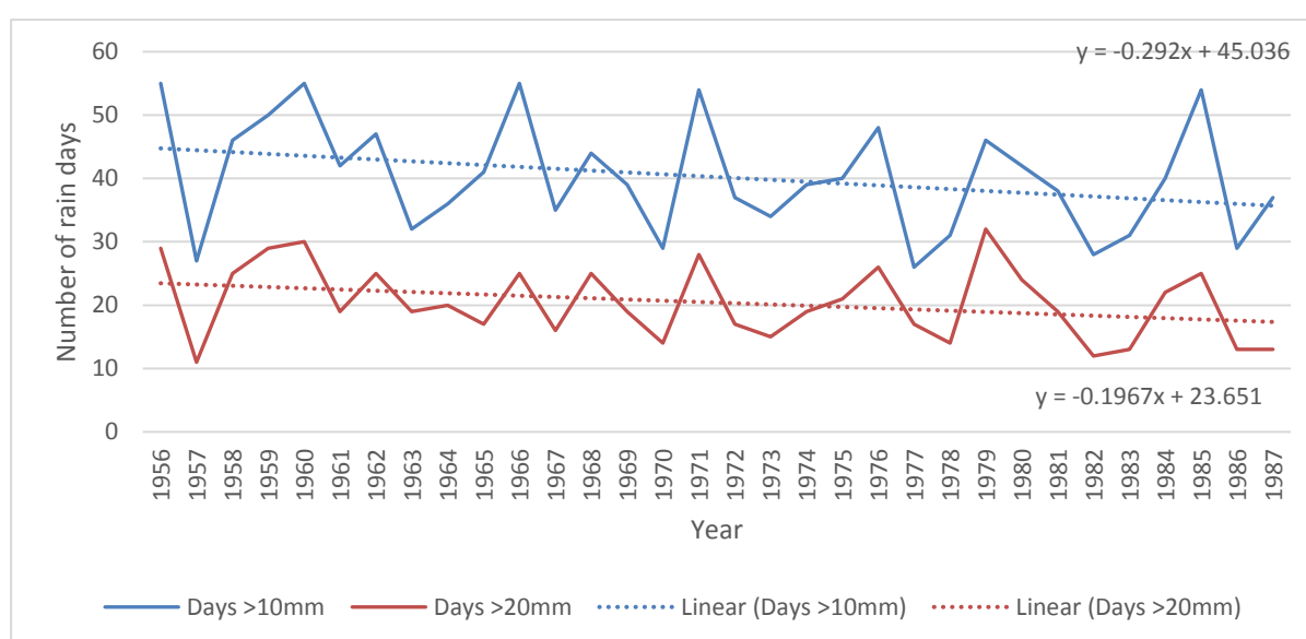
Figure 4-9: Number of days per year between 1956 and 1987 with >10mm rain and >20mm rain at Whangarei airport.
