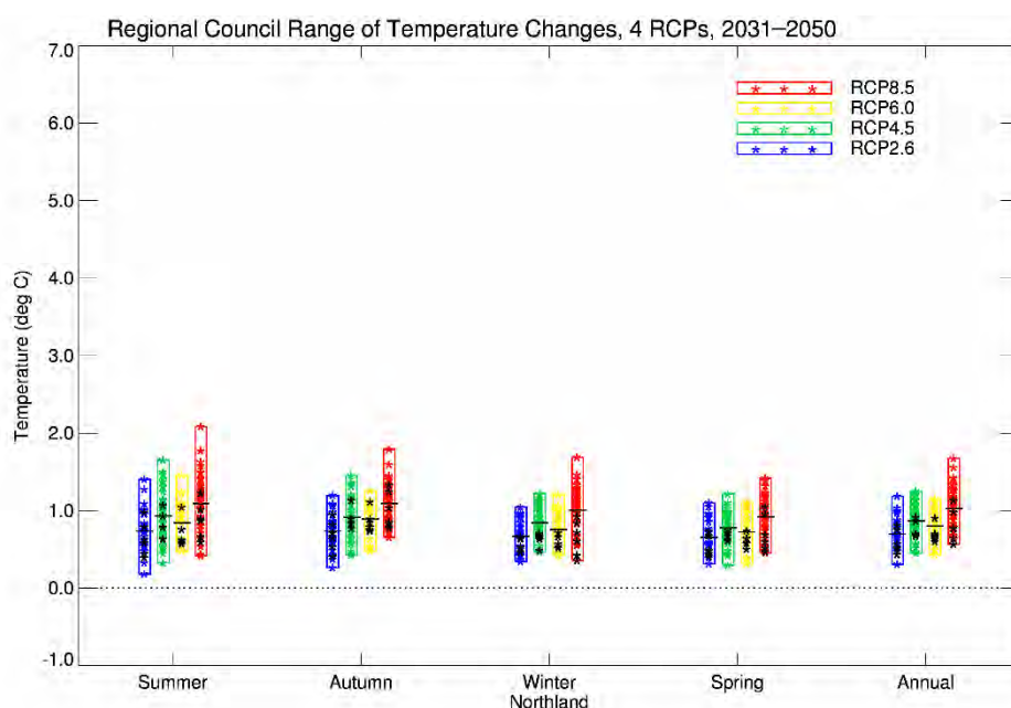
Figure 5-15: Projected seasonal temperature changes by 2040 (2031-2050) averaged over the Northland Region, for the four RCPs. The vertical coloured bars show the range over all climate models used, and coloured stars the projected changes for each model individually (results from statistical downscaling). The black stars represent the 6-model dynamical downscaling changes. The short horizontal line is the model-average warming over all statistical and dynamical models. Blue = RCP 2.6, 23 models; green = RCP 4.5, 37 models; yellow = RCP 6.0, 18 models; red = RCP 8.5, 41 models. © NIWA.
