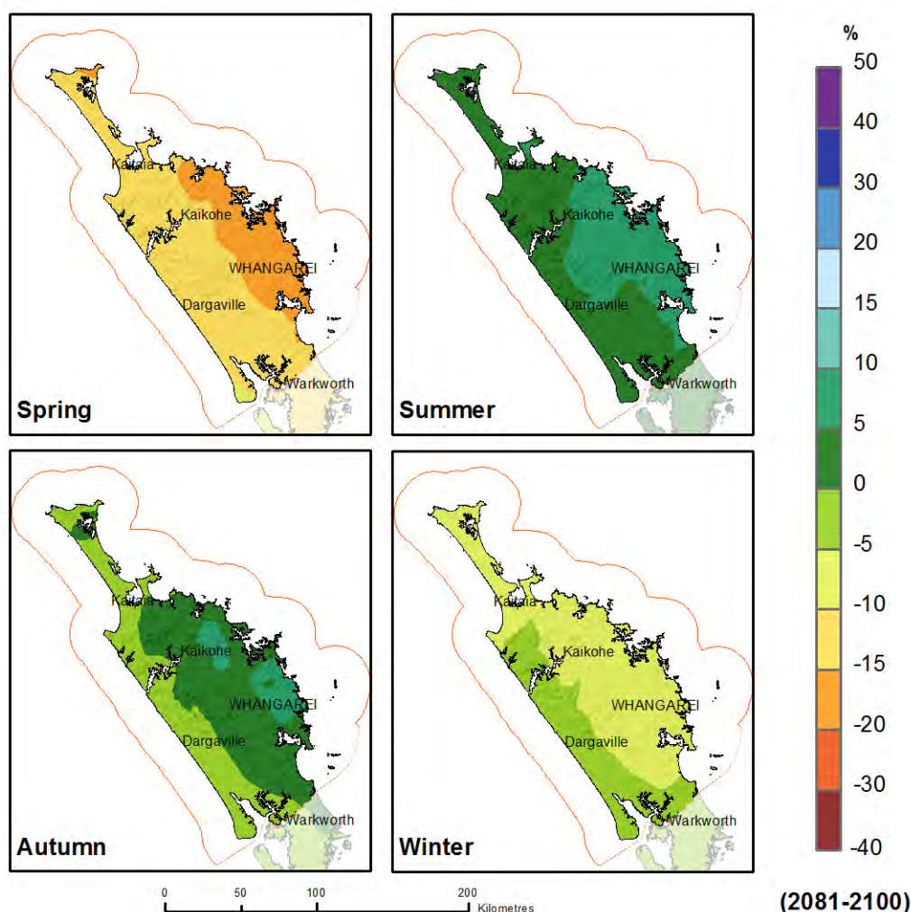
Figure 5-14: Projected seasonal precipitation changes (in %) at 2090 (2081-2100 average). Relative to 1986-2005 average, for the IPCC RCP 8.5 scenario, averaged over 41 climate models. ©NIWA.
