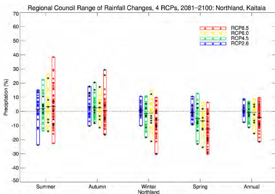
Figure 5-20: Projected seasonal rainfall changes by 2090 (2081–2100) for Kaitia for the four RCPs. The vertical coloured bars show the range over all climate models used, and coloured stars the projected changes for each model individually (results from statistical downscaling). The black stars represent the 6-model dynamical downscaling changes. The short horizontal line is the model-average rainfall over all statistical and dynamical models. Blue = RCP 2.6, 23 models; green = RCP 4.5, 37 models; yellow = RCP 6.0, 18 models; red = RCP 8.5, 41 models. © NIWA.
