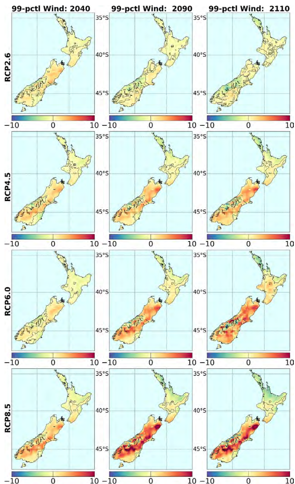
Figure 5-26: Change in the magnitude of the 99th percentile of daily-mean wind speed, for all four RCPs and three future time periods. Relative to the daily 99th percentile in the baseline 1986-2005 period. Blue and green shades indicate a decrease in wind speed and red shades indicate an increase in wind speed. After Mullan et al. (2016).
