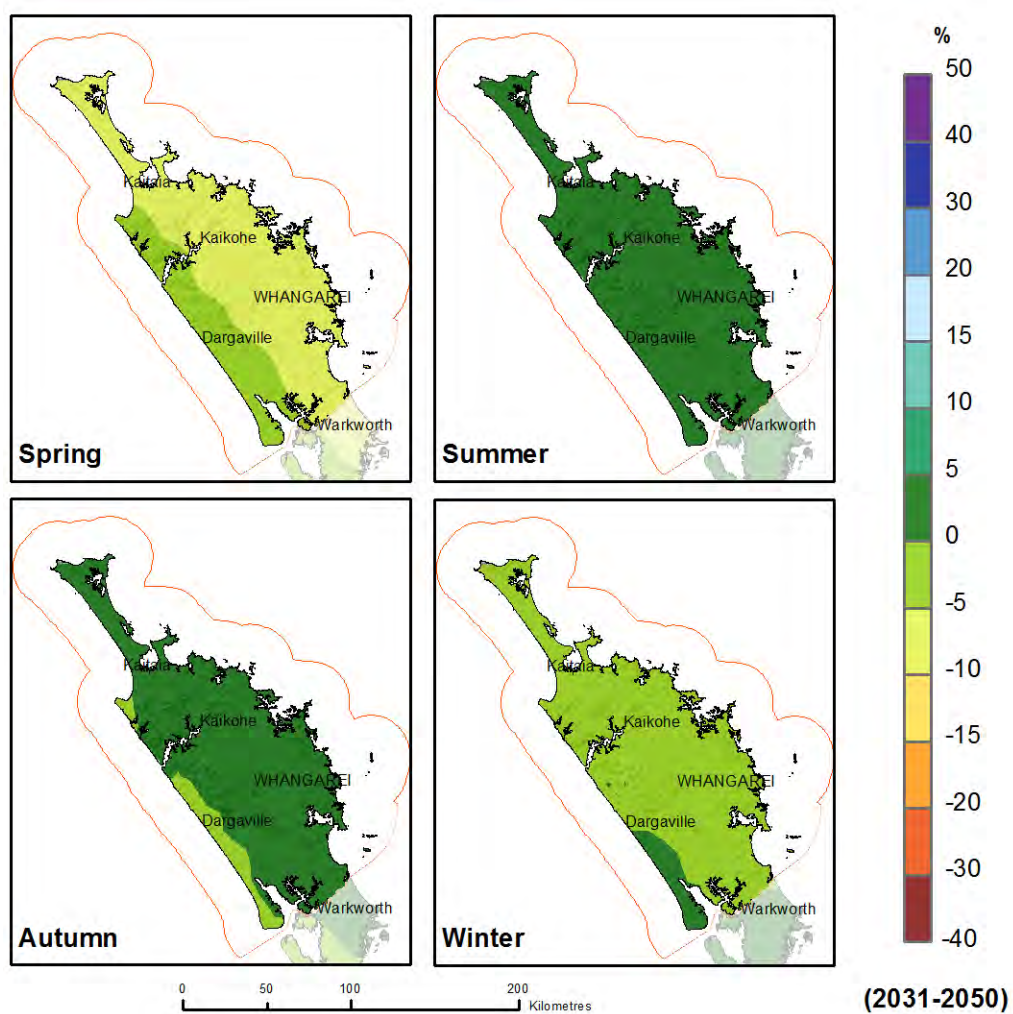
Figure 5-13: Projected seasonal precipitation changes (in %) at 2040 (2031-2050 average). Relative to 1986-2005 average, for the IPCC RCP 8.5 scenario, averaged over 41 climate models. ©NIWA.
