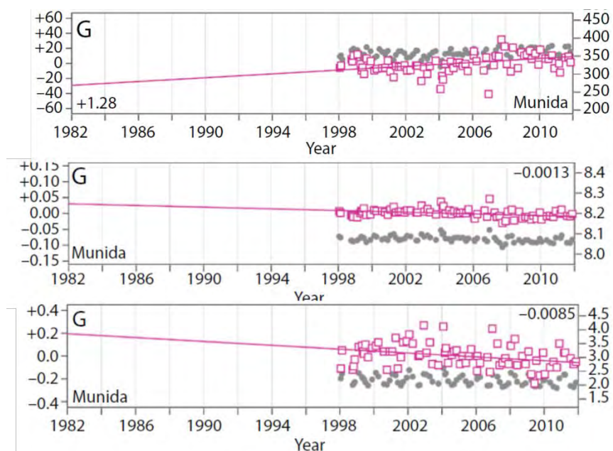
Figure 5-32: Time series of Surface seawater \text{pCO}_2 ( \mu\text{atm} , top panel), pH (middle panel), and saturation state of the carbonate mineral, aragonite (lower panel). This time series is from Sub-Antarctica water at the
