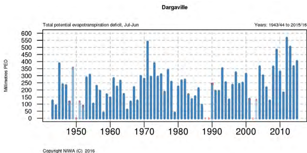
Figure 4-6: PED accumulation from 1943-2015 (July-June years) for Dargaville (combined record from agent numbers 1192, 16137, 25119). Light blue bars indicate years where there are missing data, and small red numbers indicate the amount of months in that year with full data. © NIWA.
