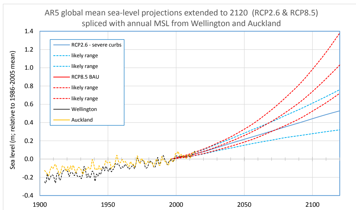
Figure 5-28: AR5 global mean sea-level projections extended to 2120 spliced with annual MSL from Wellington and Auckland. Dashed lines show the upper and lower bounds of the likely range for each RCP shown, which in the calibrated language of IPCC means there is a 33% change the SLR could lie outside those bounds (Church et al., 2013a). Source: QA for annual MSL for historic NZ ports undertaken by Prof. John Hannah and NIWA – data sourced originally from the port companies and obtained from the Land Information
