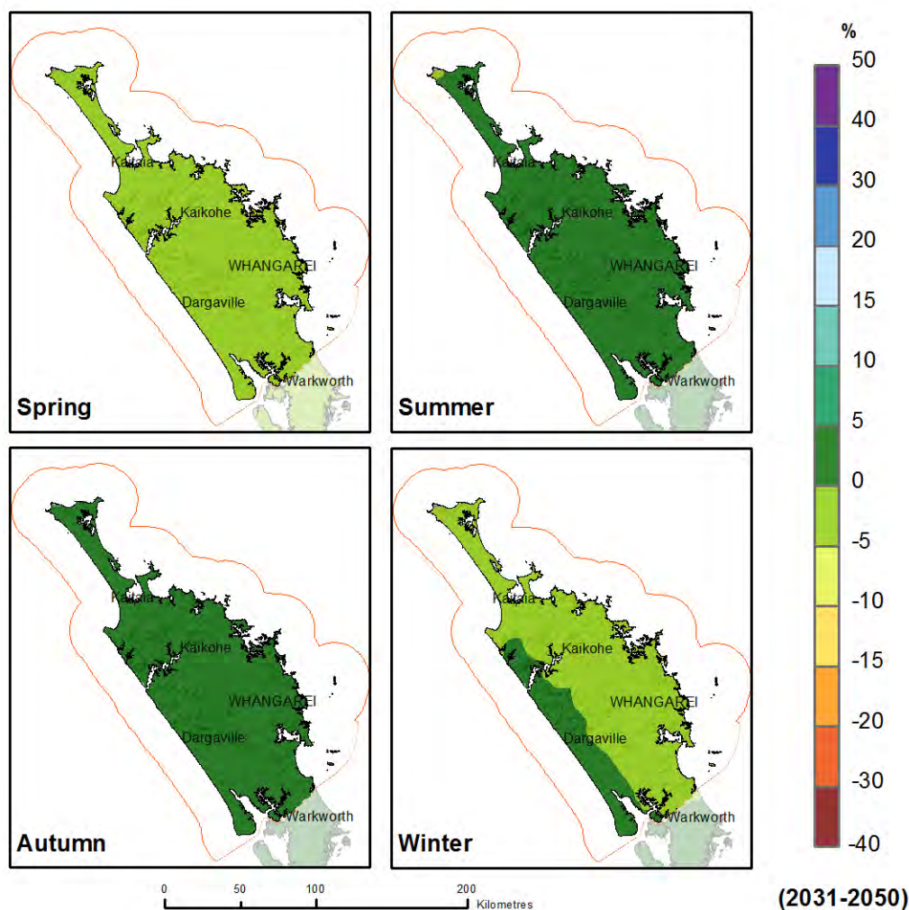
Figure 5-11: Projected seasonal precipitation changes (in %) at 2040 (2031-2050 average). Relative to 1986-2005 average, for the IPCC RCP 4.5 scenario, averaged over 37 climate models. ©NIWA.
