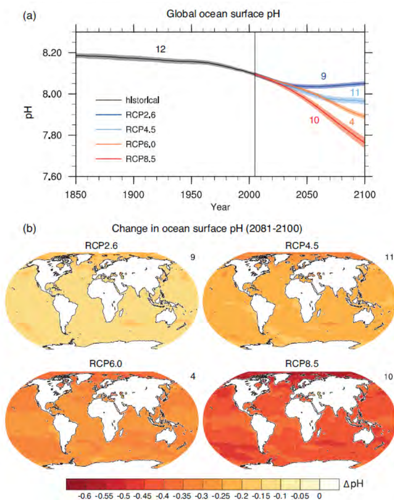
Figure 5-30: Change in ocean surface pH. Time series (model averages and minimum to maximum ranges and (b) maps of multi-model surface ocean pH for the scenarios RCP2.6, RCP4.5, RCP6.0 and RCP8.5 in 2081-2100. The maps in (b) show change in global ocean surface pH in 2081-2100 relative to 1986-2005. The number of CMIP5 models to calculate the multi-model mean is indicated in the upper right corner of each panel. Figure after (IPCC, 2013).
