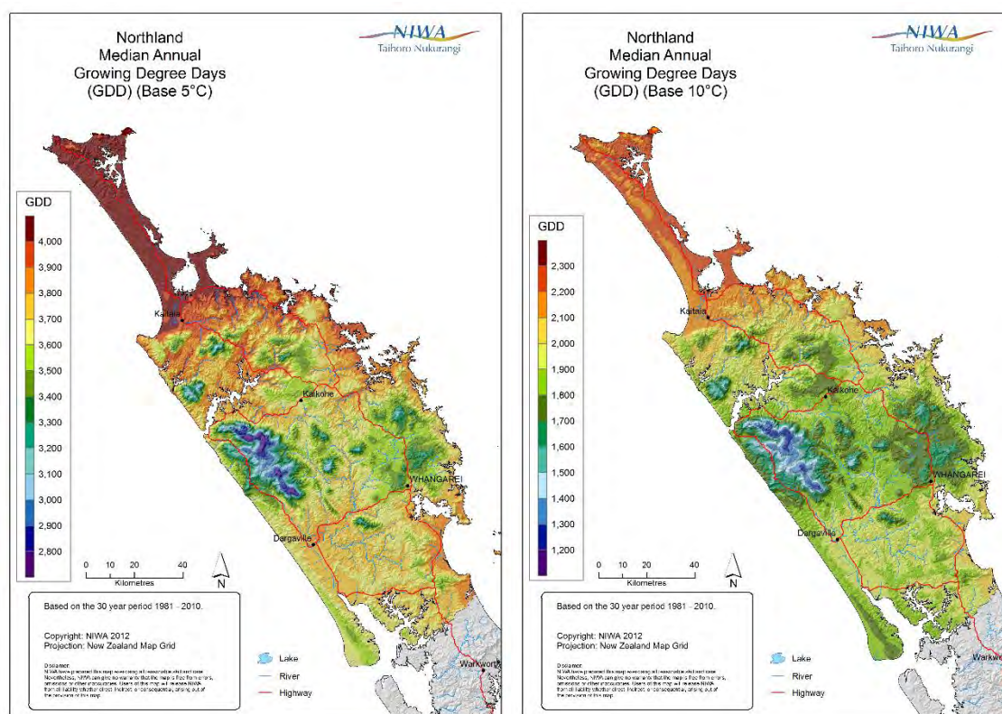
Figure 4-10: Median annual growing degree-days in Northland Region, 1981-2010. Left: Base 5°C, Right: Base 10°C. Note the change in scale between the figures. © NIWA.
