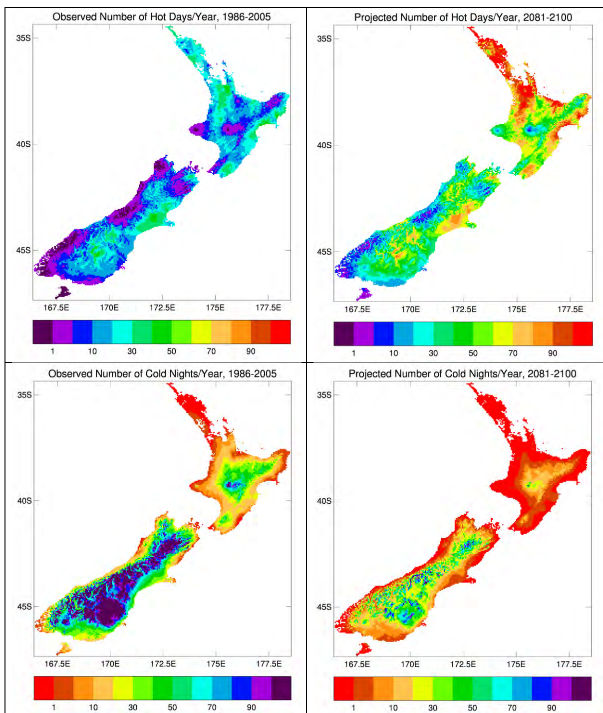
Figure 5-10: Number of days per year of "hot days" (maximum temperature of 25°C or above, top row) and "cold nights" (minimum temperature of 0°C or below, bottom row): 'current' climate (1986-2005), left; 2090 climate under RCP8.5 (right). After Mullan et al. (2016).
