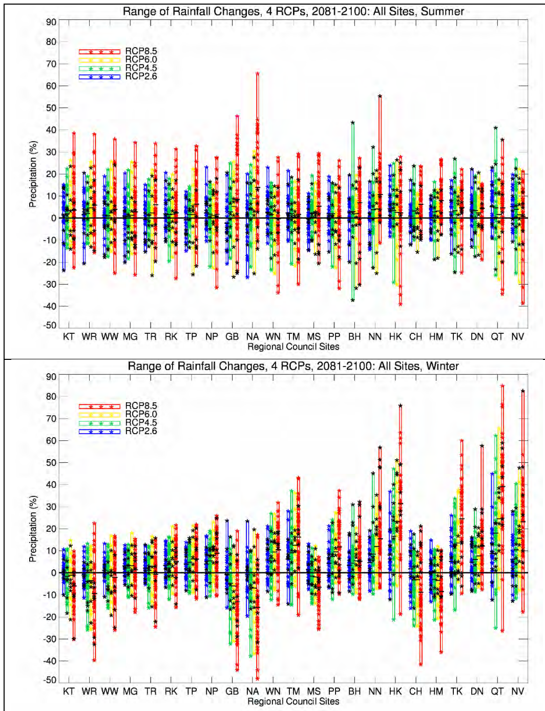
Figure 5-22: Projected precipitation changes for selected sites within all Regions for 2090, for summer (top panel) and winter (bottom panel) seasons, for all RCPs (bars) and all models. Coloured stars refer to statistical downscaling, whereas the black stars correspond to the 6-model RCM-downscaling. The sites chosen (and Regions) are: Kaitiaki [KT] and Whangarei [WR] (Northland), Warkworth [WW] and Mangere [MG] (Auckland), Tauranga [TR] (Environment Bay of Plenty), Ruakura [RK] and Taupo [TP] (Waikato), New Plymouth [NP] (Taranaki), Gisborne [GB] (Gisborne), Napier [NA] (Hawkes Bay), Wanganui [WN] and Taumarunui [TM] (Horizons Manawatu-Wanganui), Masterton [MS] and Paraparaumu [PP] (Wellington), Blenheim [BH] (Marlborough), Nelson [NN] (Tasman), Hokitika [HK] (West Coast), Christchurch [CH], Hanmer [HM] and Tekapo [TK] (Canterbury), Dunedin [DN] and Queenstown [QT] (Otago), and Invercargill [NV] (Southland). After Mullan et al. (2016).
