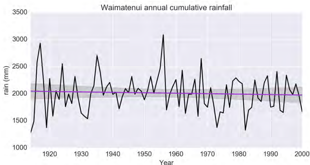
Figure 4-4: Annual rainfall total (mm) at Waimatenui (south of Kaikohe) from 1914 to 2000. The purple line removes the year-to-year variability and shows a long term flat trend. © NIWA.
