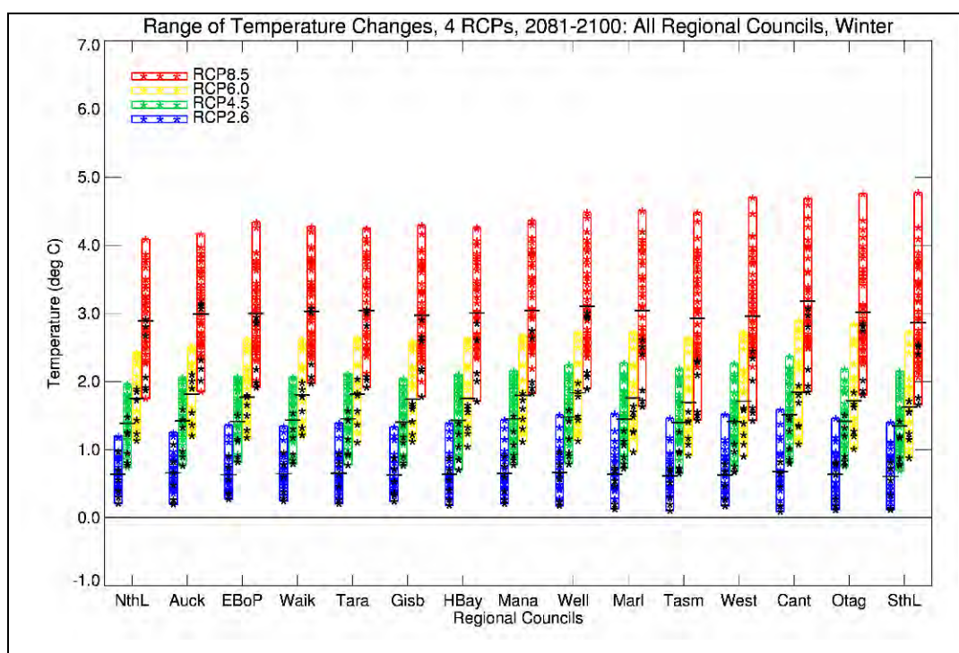
Figure 5-7: Projected temperature changes for all Regional Council area for 2090, for summer (top panel) and winter (bottom panel) seasons, for all RCPs (bars) and all models (coloured stars), as derived by statistical downscaling. The black stars correspond to the 6-model RCM-downscaling. The Regional Council abbreviations (in order) represent: Northland, Auckland, Environment Bay of Plenty, Waikato, Taranaki, Gisborne, Hawkes Bay, Horizons Manawatu-Wanganui, Wellington, Marlborough, Tasman (including Nelson City), West Coast, Environment Canterbury, Otago, and Southland. After Mullan et al. (2016).
