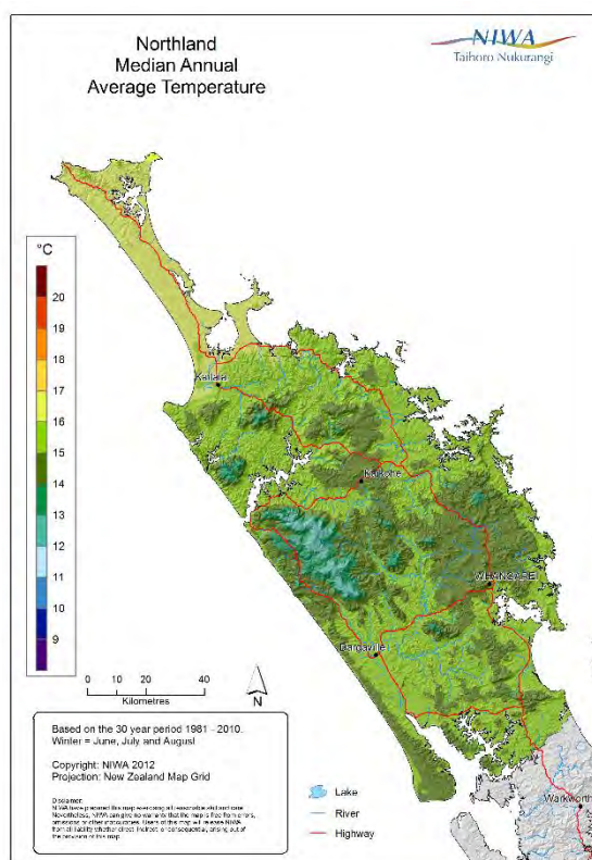
Figure 4-1: Annual average temperature for the Northland region (median for 1981-2010). ©NIWA.
